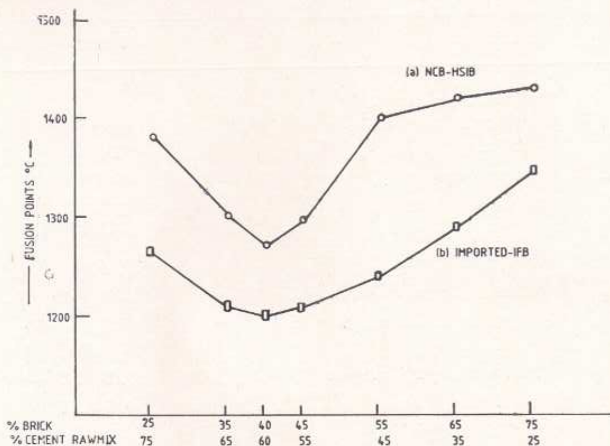
Fig 2 Relationship between fusion points of mixtures of (a) Cement raw mix + NCB-HSIB and (b) Cement raw mix + imported IFB studied under Leitz heating microscope
