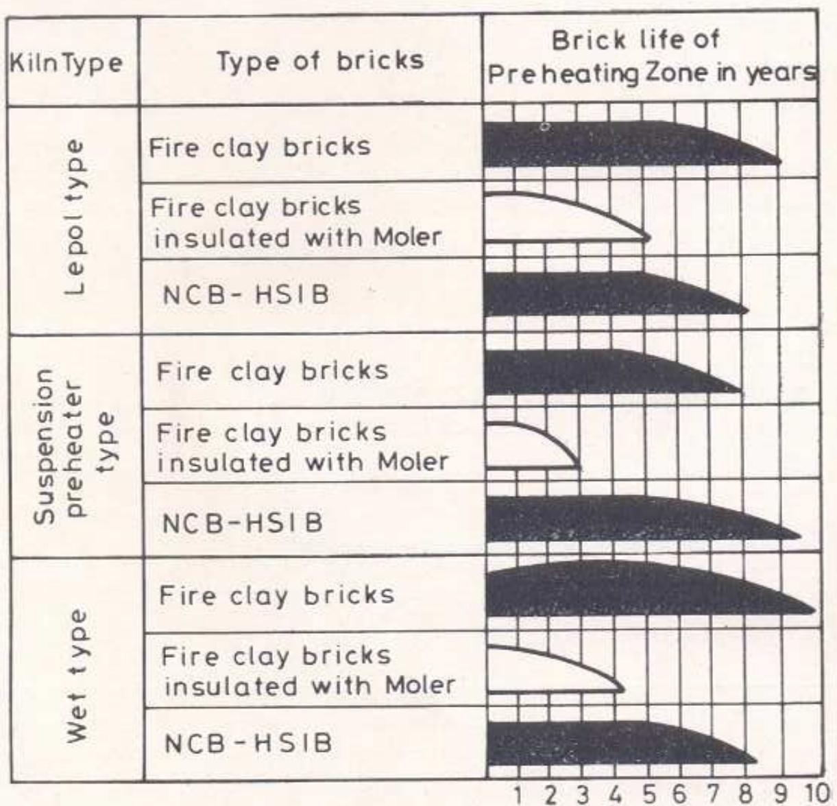
Fig 3 Expected life of NCB High Strength Insulating Bricks in comparison to other bricks
