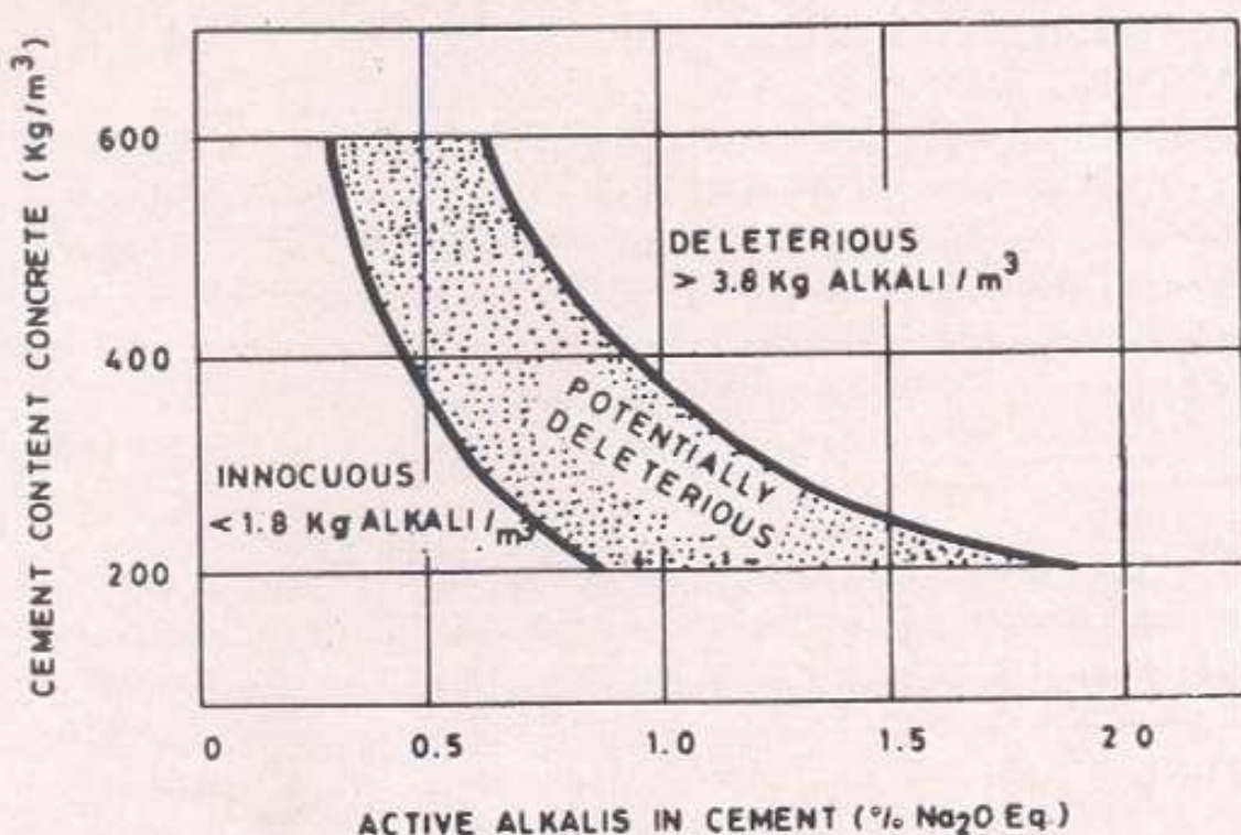
Fig 1 . Schematic relationship between alkali content of cement and total cement content in concrete to prevent ASR
